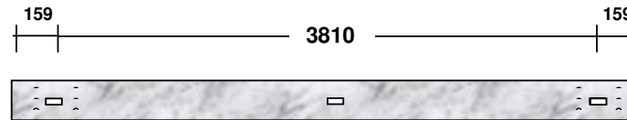
Standard Length Highway Rail. Effective cover 3.810m Lap in direction of traffic
