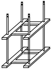
Hold Down Cage for poles up to 12.0m
